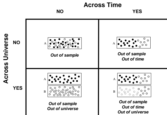
FIGURE 4 Schematic of out of sample validation techniques
