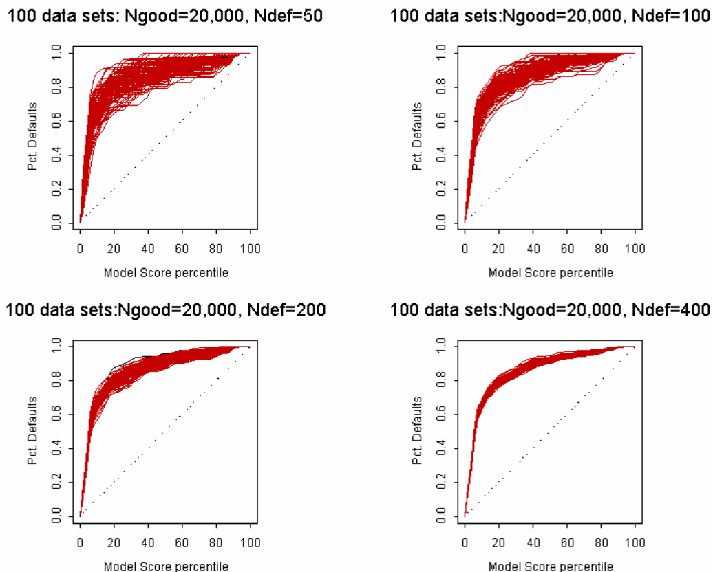
FIGURE 6 Variability of test results when different numbers of defaults are used for evaluation These graphs show the results of evaluating a simple model using randomly selected samples of varying numbers of defaults. Each figure shows 100 CAP pots, each of which is based on evaluating the same model using a different sample of 20,000 non-defaulting observations and 50, 100, 200, and 400 defaulting observations.
