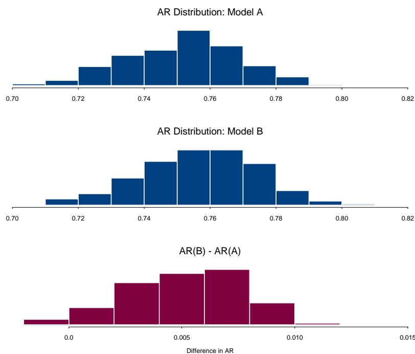
FIGURE 9 Bootstrap results of individual vs. matched samples
