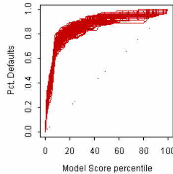
100 data sets: Ngood=50,000, Ndef=100
