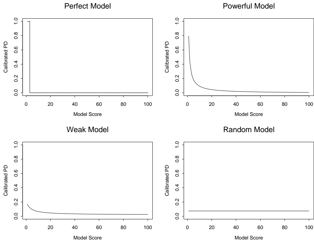
FIGURE 3 Calibration curves for four hypothetical models with different power
