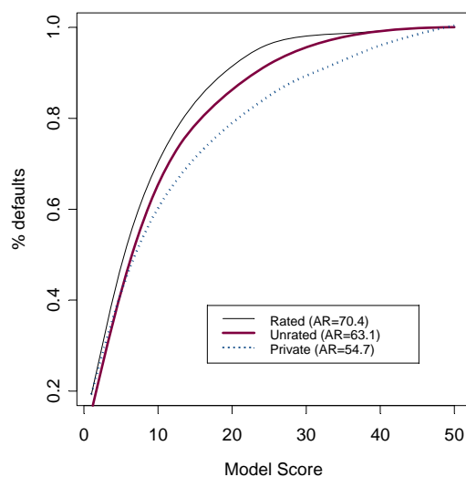
FIGURE 10 Same model applied to rated, unrated and private firms
