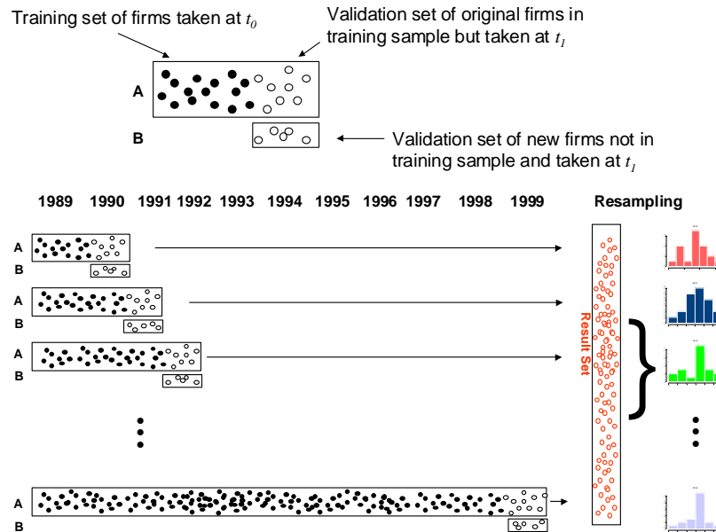
FIGURE 5 Schematic of walk-forward testing approach
