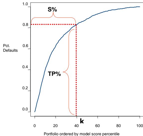
FIGURE 12 A schematic representation of a CAP plot
