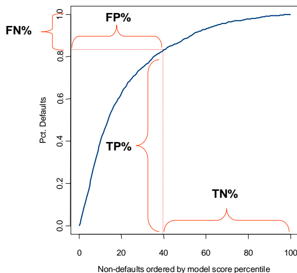
FIGURE 1 Schematic of a ROC
