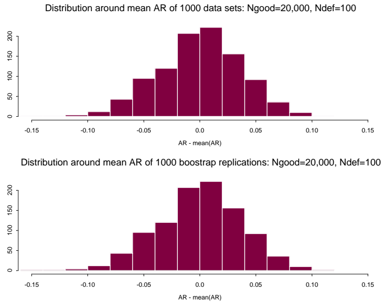
FIGURE 8 Two similar distributions of ARs: 1000 samples and a bootstrap distribution for a single sample Top frame: Distribution of Accuracy Ratios for 1000 samples from data set of defaulted and non-defaulted firms. Each set contains 20,000 non-defaulted observations and 100 defaulted observations. Bottom frame: Distribution of Accuracy Ratios for 1000 bootstrap replications of a single sample of 100 defaults and 20,000 non-defaults. Results adjusted to a mean of zero to facilitate direct comparison.
