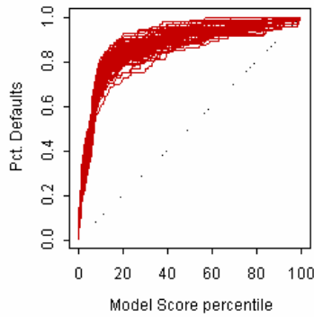
100 data sets: Ngood=20,000, Ndef=100
