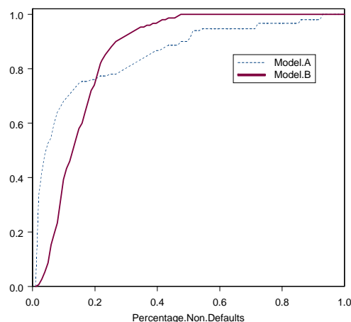
FIGURE 2 Two ROCs with the same area but different shapes
